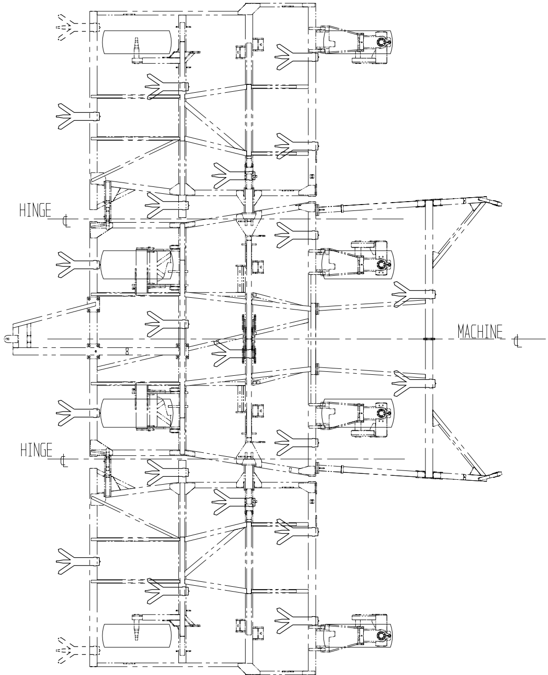
Ag-Boss - 8m - 400mm Tyne Spacing
