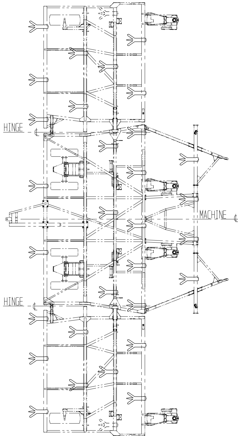
Ag-Boss - 12m - 2 & 4m Wheel Centres - 400mm Tyne Spacing
