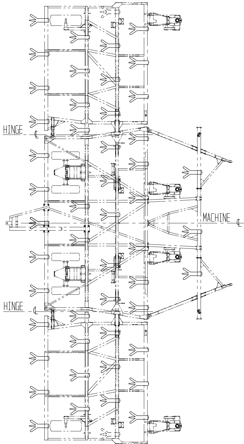
Ag-Boss - 12m - 2 & 4m Wheel Centres - 250mm Tyne Spacing
