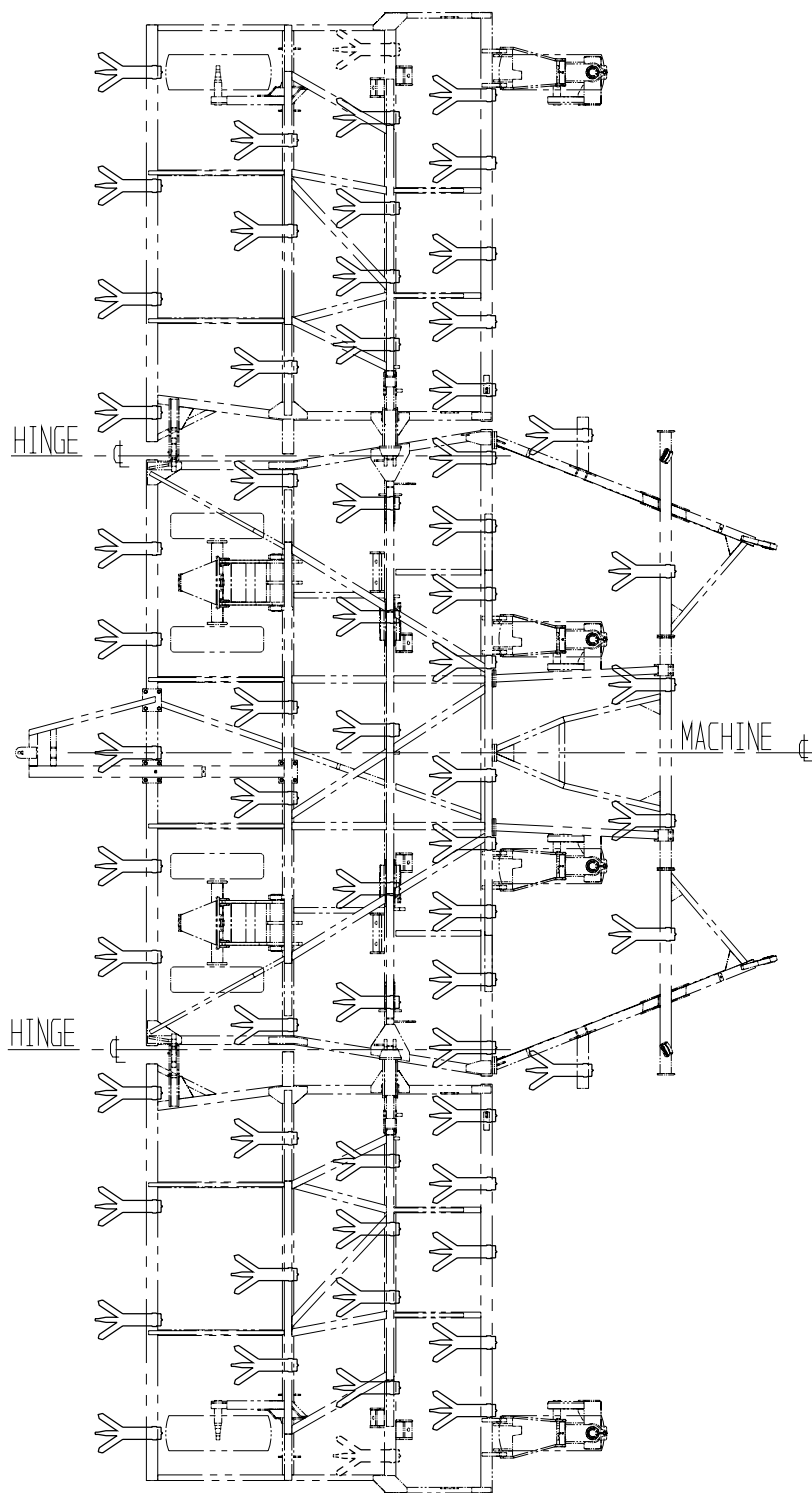
Ag-Boss - 12m - 2 & 4m Wheel Centres - 200mm Tyne Spacing
