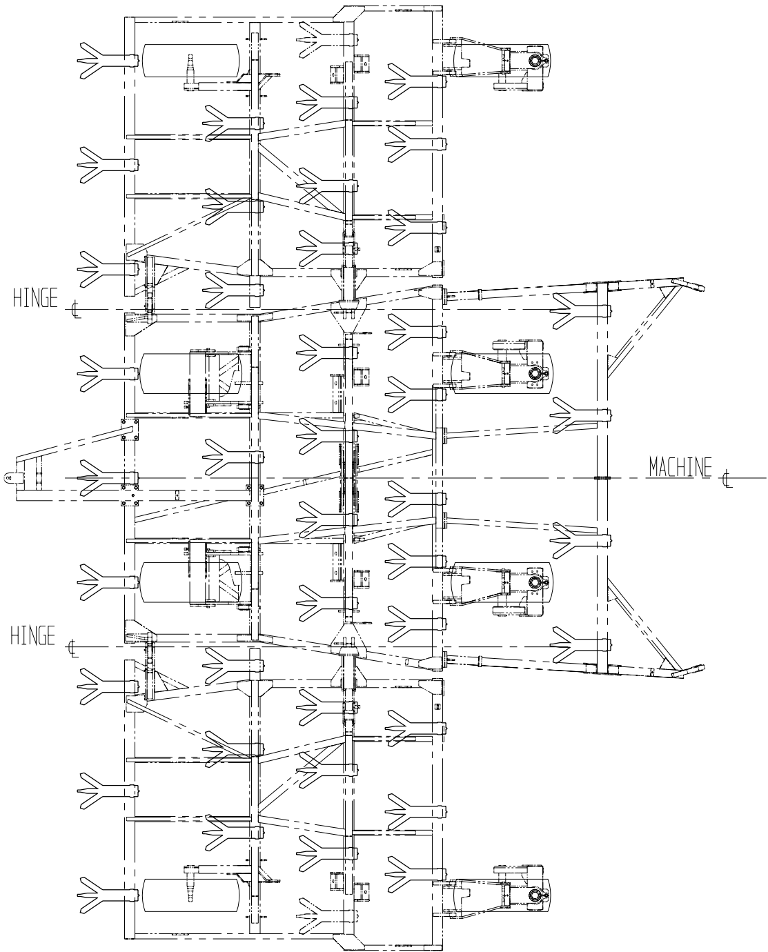
Ag-Boss - 8m - 200mm Tyne Spacing
