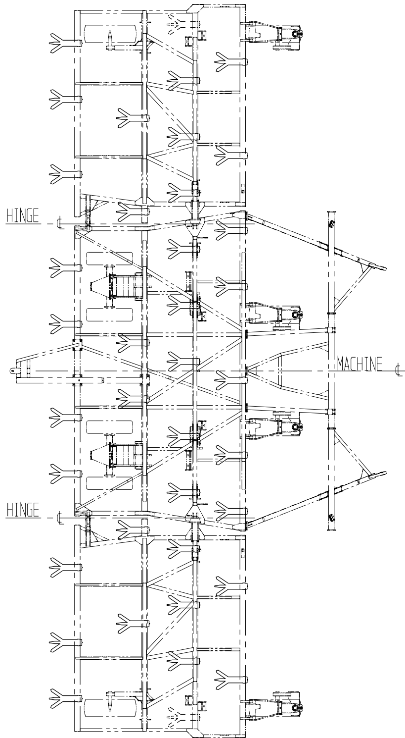
Ag-Boss - 12m - 2 & 4m Wheel Centres - 333mm Tyne Spacing
