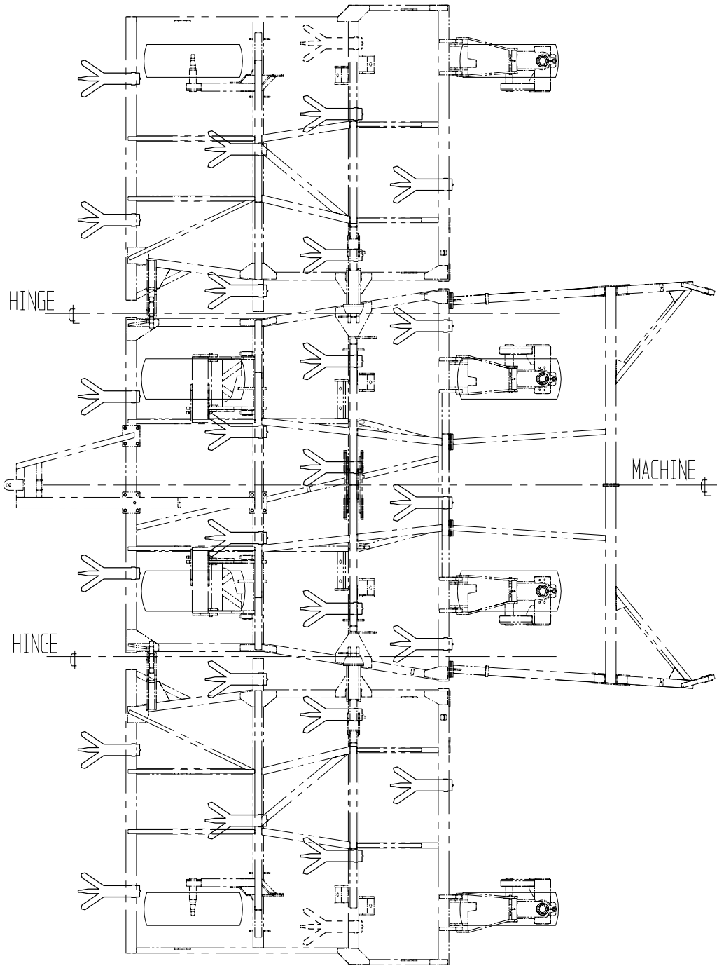
Ag-Boss - 8m - 333mm Tyne Spacing
