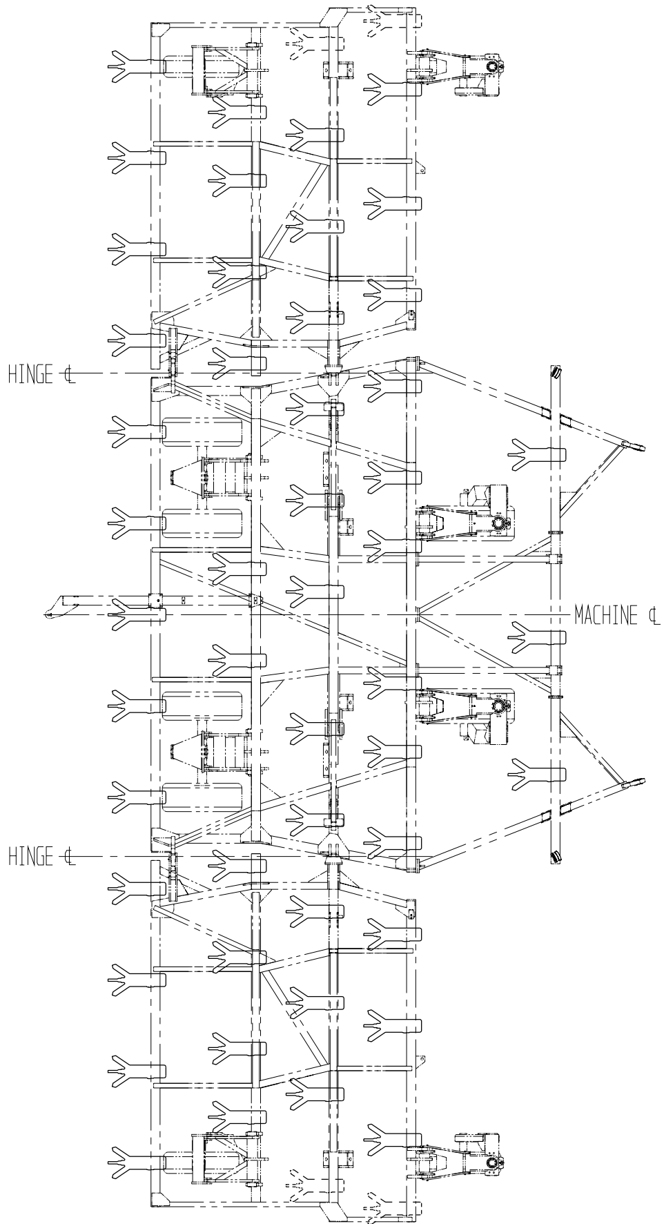
Penetrator - 12m - 2 & 4m Wheel Centres - 250mm Tyne Spacing
