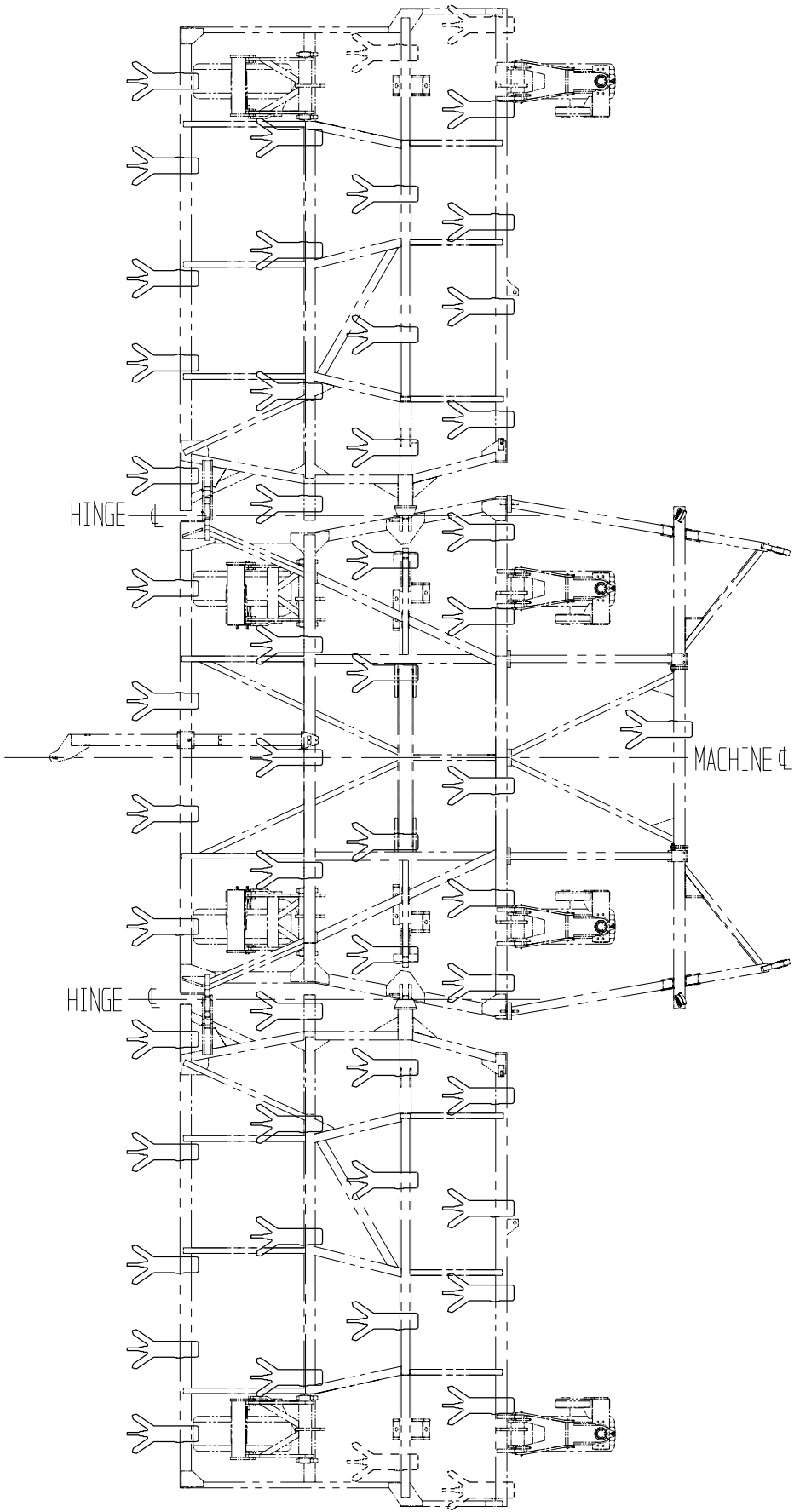
Penetrator - 12m - 3m Wheel Centres - 250mm Tyne Spacing
