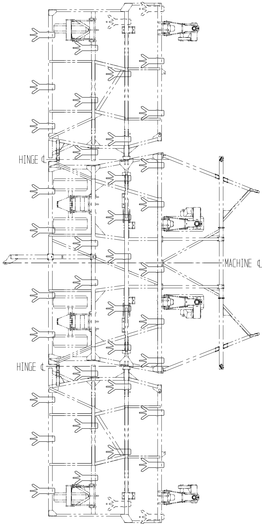
Penetrator - 12m - 2 & 4m Wheel Centres - 333mm Tyne Spacing
