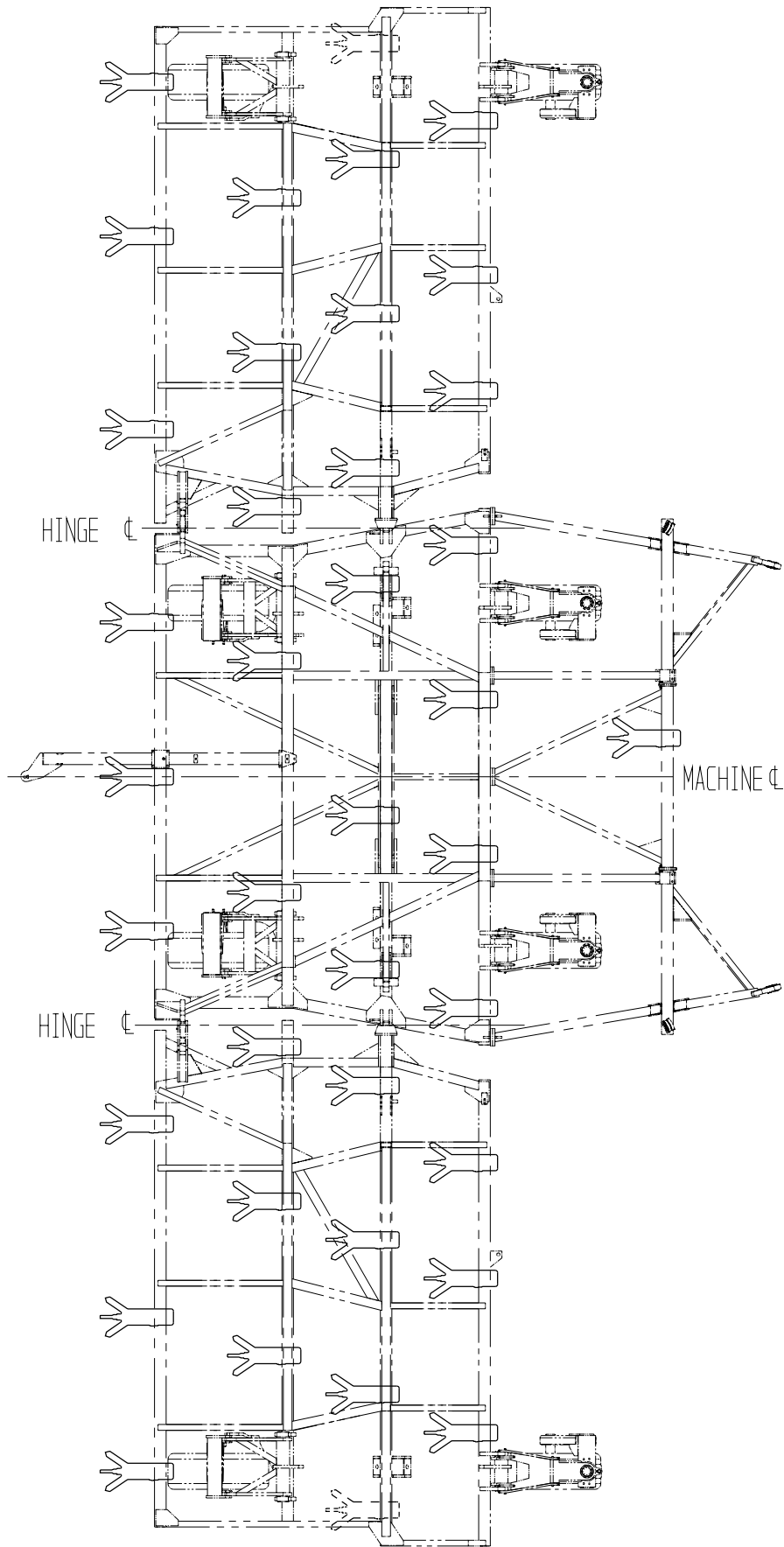
Penetrator - 12m - 3m Wheel Centres - 333mm Tyne Spacing
