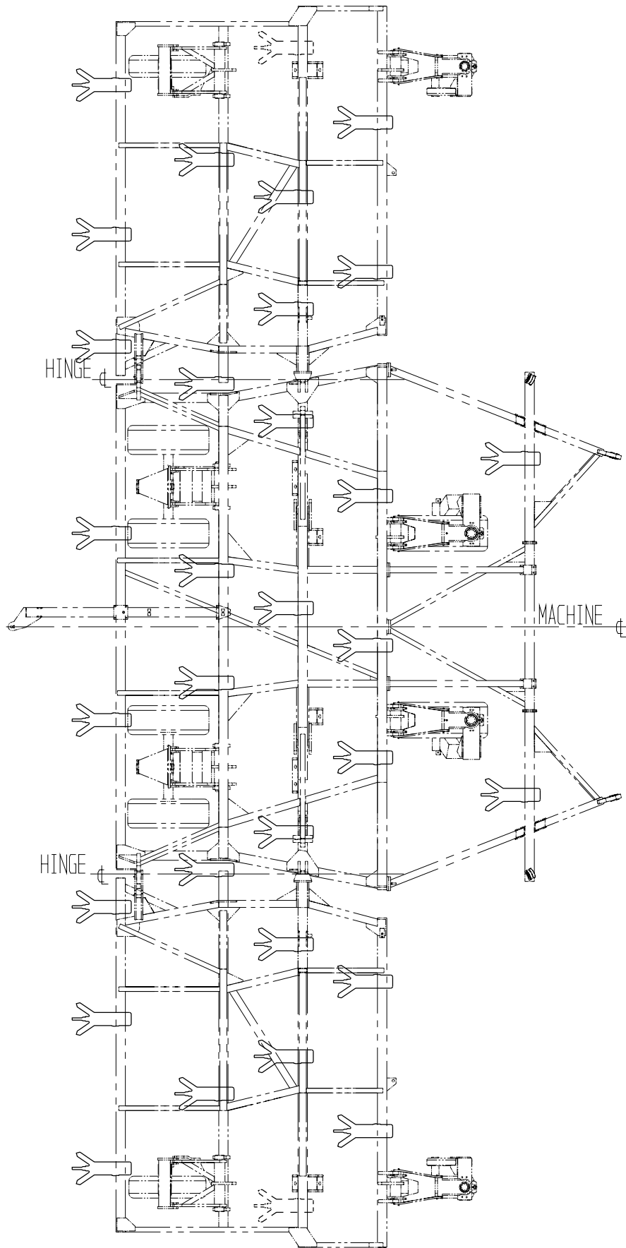
Penetrator - 12m - 2 & 4m Wheel Centres - 400mm Tyne Spacing
