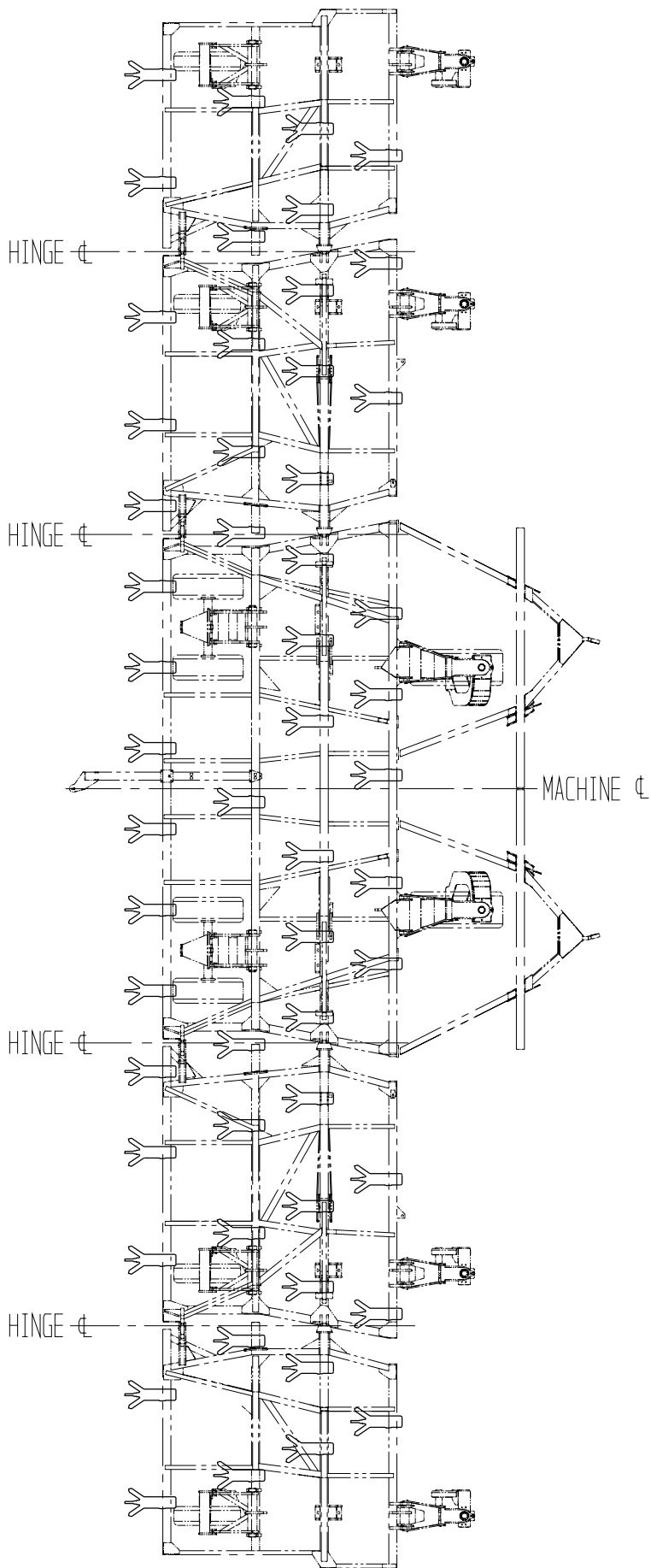
Penetrator - 18m - 3 & 5m Wheel Centres - 333mm Tyne Spacing
