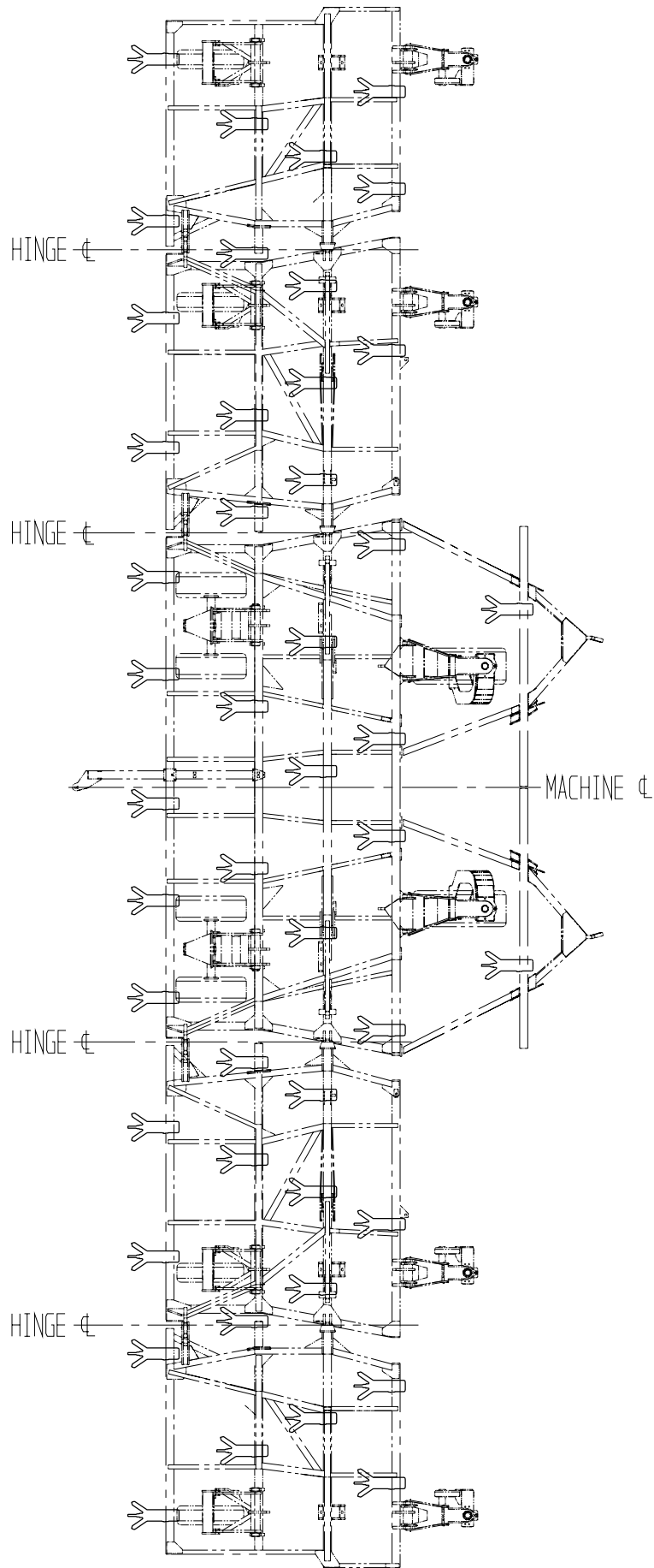
Penetrator - 18m - 3 & 5m Wheel Centres - 400mm Tyne Spacing
