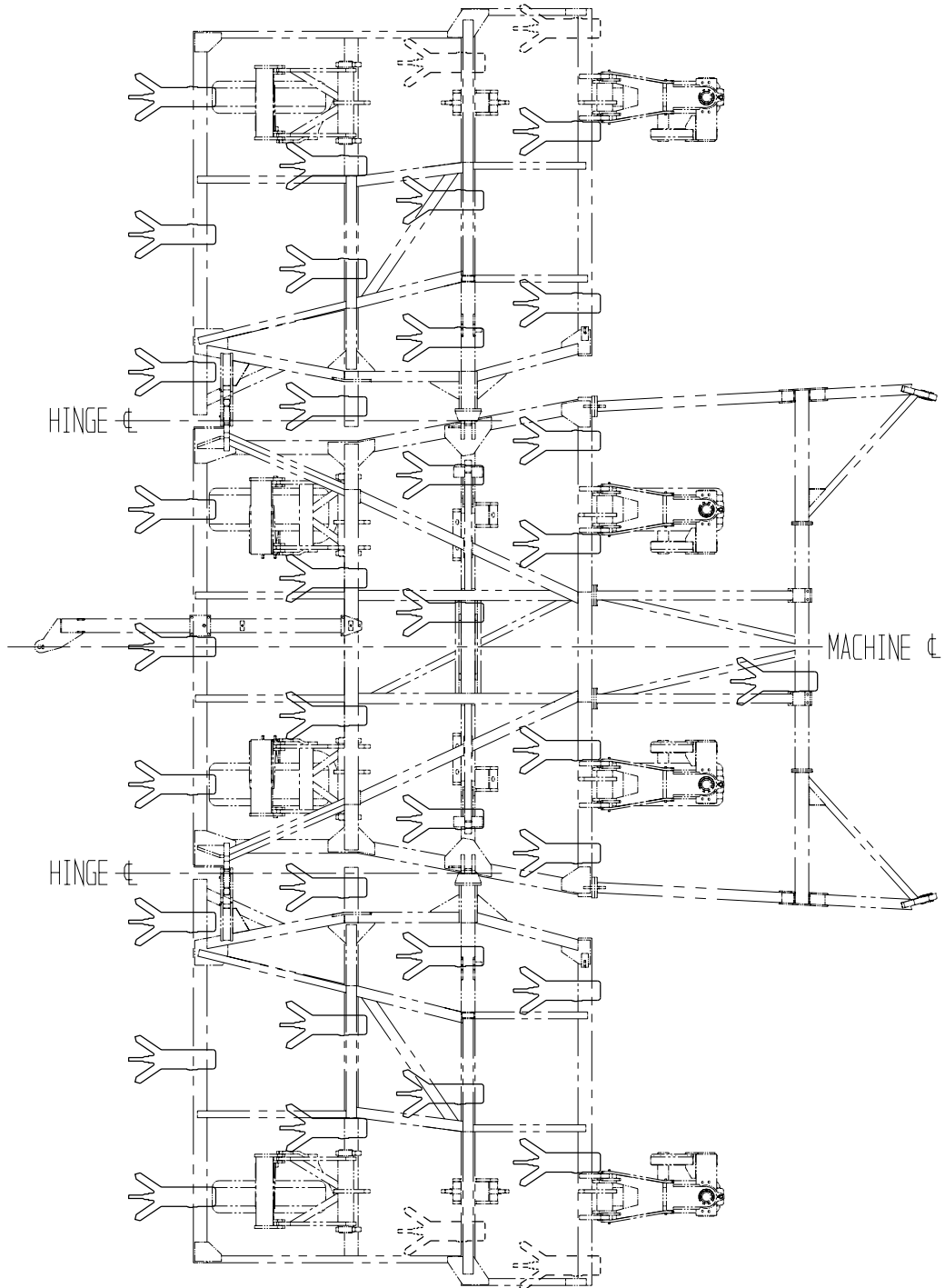
Penetrator - 8m - 250mm Tyne Spacing
