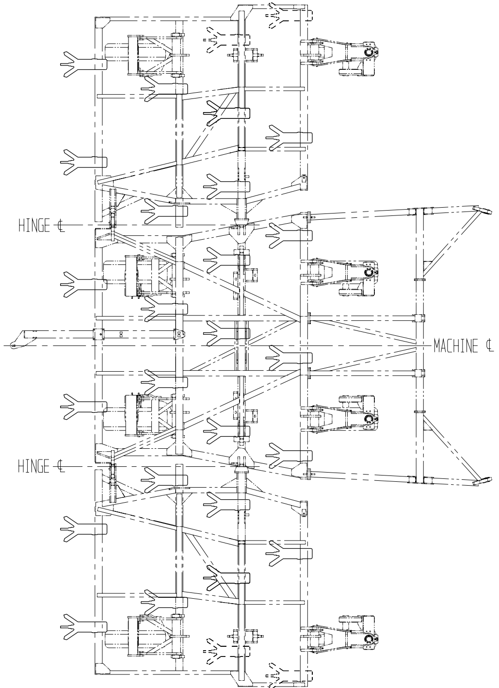
Penetrator - 8m - 333mm Tyne Spacing
