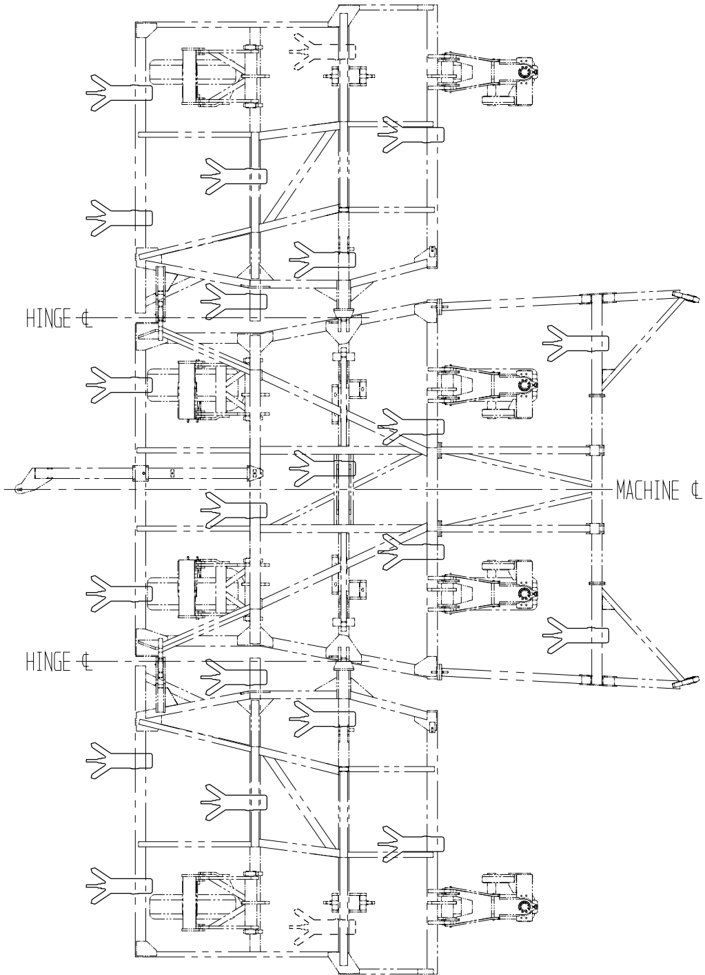
Penetrator - 8m - 400mm Tyne Spacing
